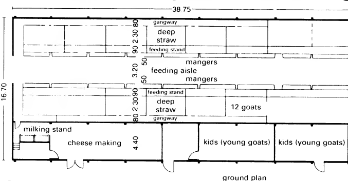
13 Twin-room deep pen
